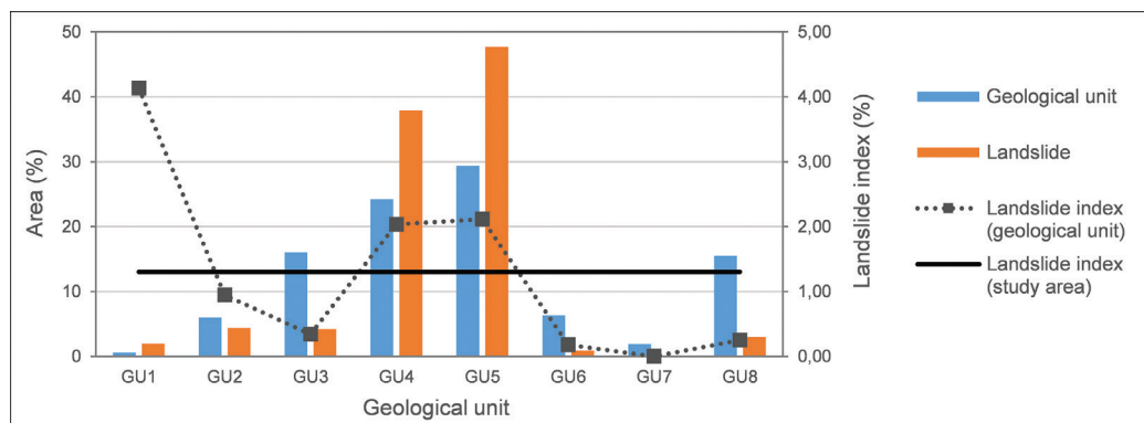
Figure 6. Landslide area distribution in different geological units (GU1 – Limestones and marls (Badenian); GU2 – Clayey limestones and marls (Early - Late Pannonian); GU3 – Marls with sandy interlayers (Late Pannonian); GU4 – Sands with silts and gravel interlayers (Late Pannonian); GU5 – Clay, sands, gravels, and coal (Pliocene); GU6 – Loes (Pleistocene); GU7 – Deluvial sediments (Holocene); GU8 – Alluvial gravels, sands, and clay Holocene). The landslide index for each geological unit and for the study area is presented.
