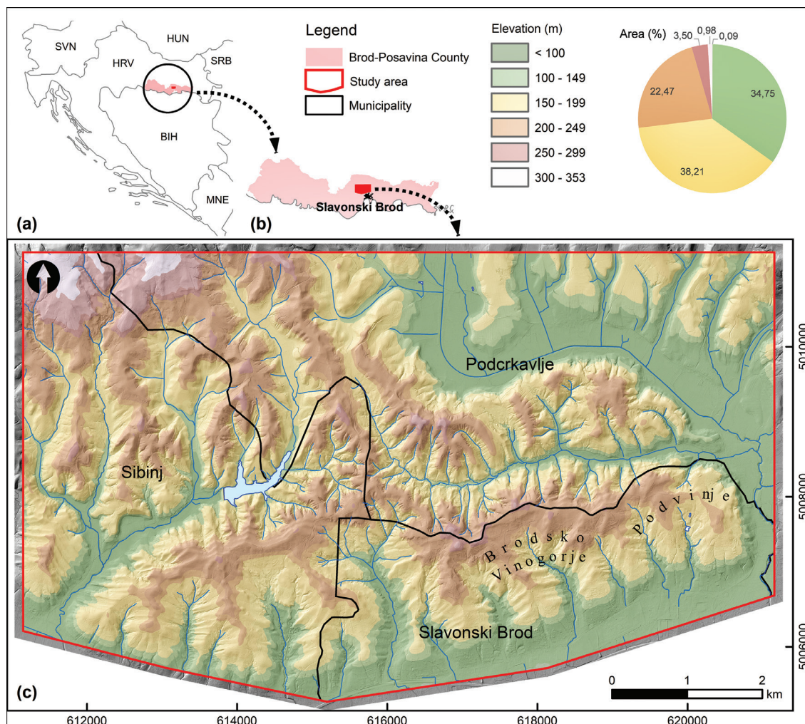
Figure 1. Location map of the study area: Brod-Posavina County in Croatia (a); the study area northwest of the City of Slavonski Brod (b); elevation map derived from LiDAR DTM and drainage network obtained from the 1:25,000 topographic map (c).
