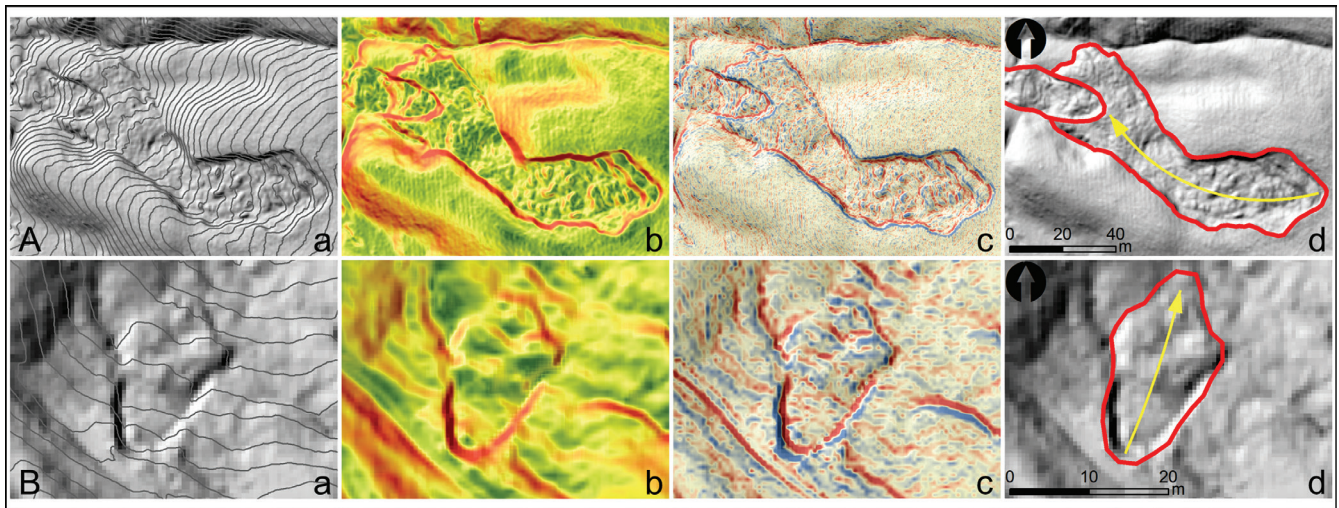
Figure 3. Examples of landslide polygon delineation for high landslide outline confidence level (A) and moderate landslide outline confidence level (B), using DTM derivatives: contour line map over the hillshade map (a); hillshade map with the transparency of 60 % over the slope map (b); hillshade map with the transparency of 60 % over the profile curvature map (c); landslide polygon on the hillshade map with movement direction (d).
