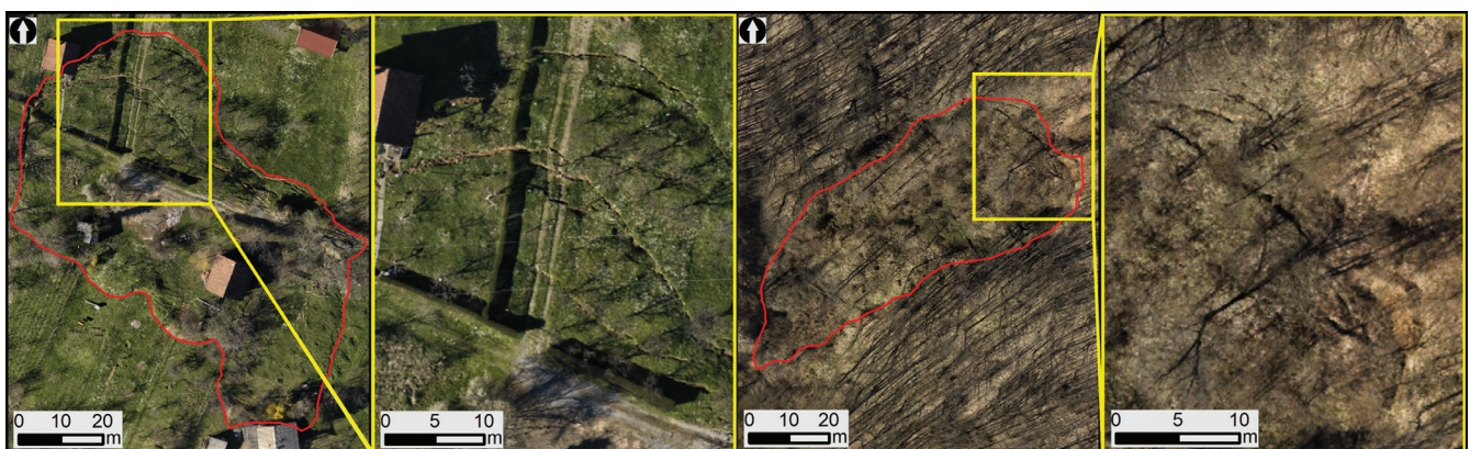
Figure 4. Visibility of landslide characteristics on HR orthophotos: landslide main scarp with several minor scarps (a); landslide main scarp and crown cracks (b).
