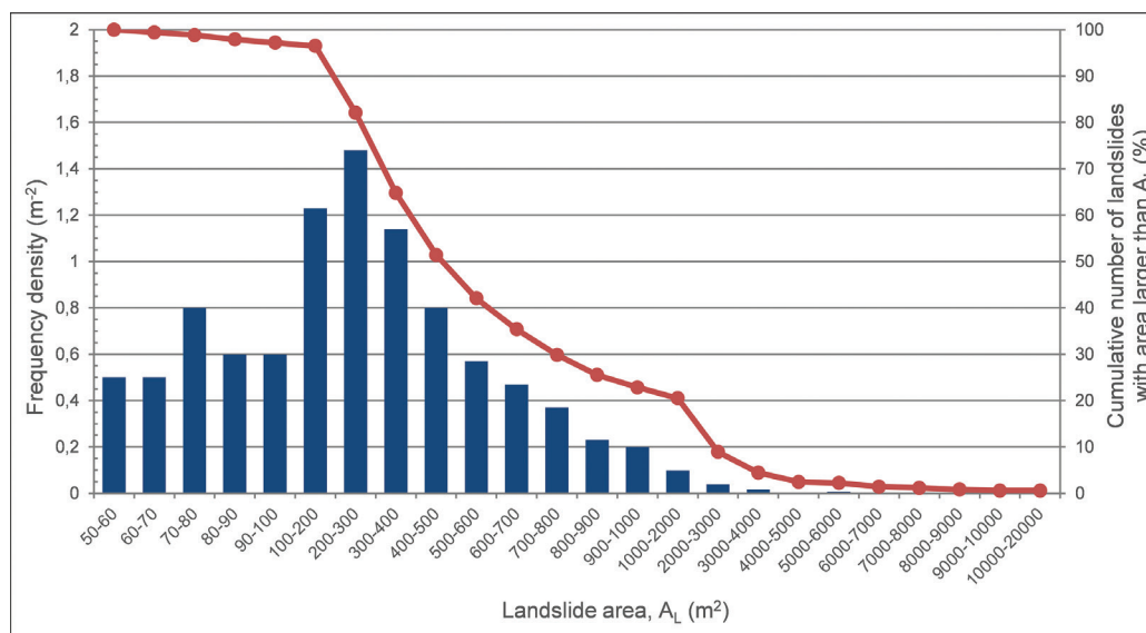
Figure 5. Frequency density and cumulative number of landslides considering landslide area.
