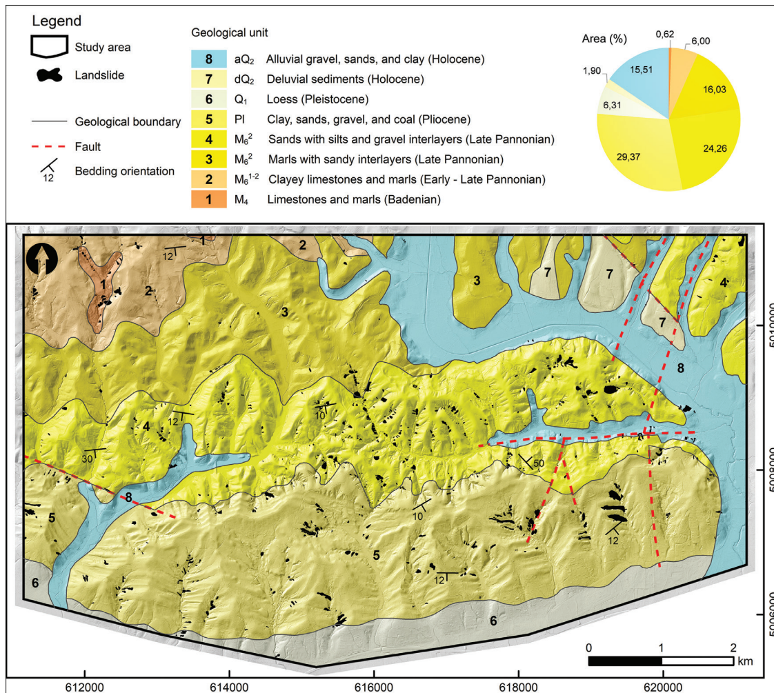
Figure 2. Geological map of the study area modified according to 1:100,000 scale basic geological maps (ŠPARICA et al., 1979a; ŠPARICA, 1986), with landslide inventory.
