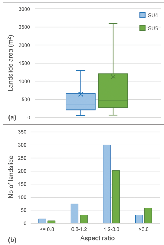
Figure 9. Area (a) and aspect ratio (b) for landslides within geological units 4 and 5.
