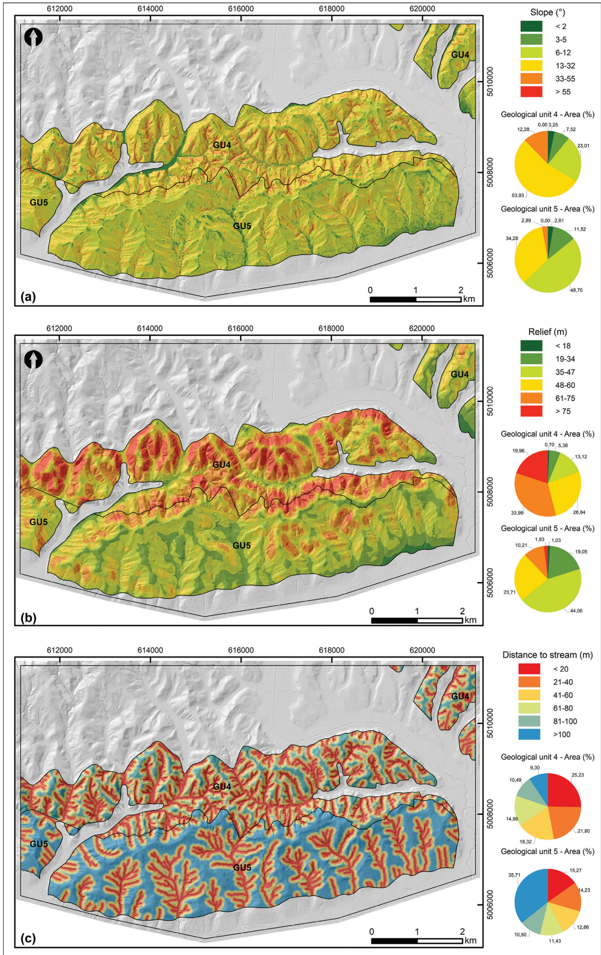
Figure 7. Spatial distribution of parameters' classes within geological units 4 and 5, concerning: slope (a); relief (b); and distance to streams (c).
