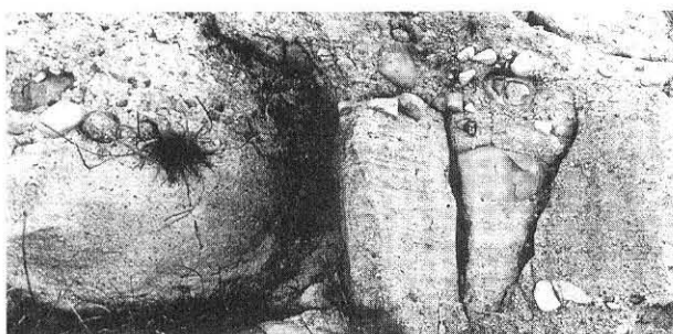
Fig. 20 In the lower part of the photograph there is a horizontally stratified granule conglomerate (visible thickness=20 cm) of probable beachface/uppermost shoreface setting. The conglomerate contains scattered pebbles in its lower part and a cobble in its upper portion. This conglomerate is overlain by cross-bedded conglomerate to granule sandstone (dipping right) inferred to have originated by a longshore migrating bedform. Locality 8 in Fig. 3.
