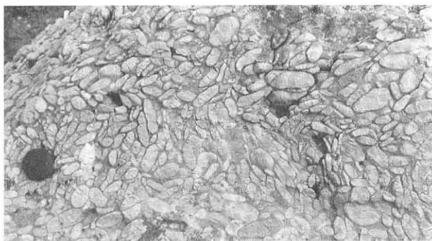
Fig. 14 "Imbricate-disc" conglomerates of the beachface. Bedding is gently inclined to the right. Two adjacent beds show oppositely dipping imbrication, and the lower bed displays imbrication in opposite directions occurring laterally. The imbrication is locally very steep. Note the sand matrix and well-sorted and rounded clasts. Lens cap is 5.8 cm in diameter. Locality 1 in Fig. 3.
