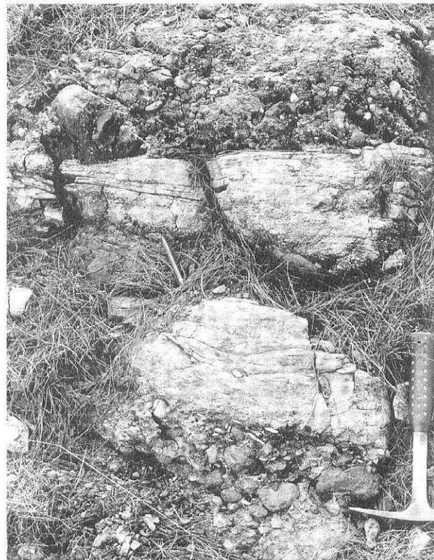
Fig. 12 Conglomerate-sandstone couplets (CS) shown by log in Fig. 11. The sandstone below the hammer is erosionaly overlain by conglomerate, which grades upwards into a finer-grained conglomerate with large nummulites (white, up to 3 cm in diameter), and then into HCS sandstone (2 in Fig. 11). This sandstone is erosionaly overlain by the next couplet (3 in Fig. 11) consisting of conglomerate (poorly exposed, marked by 13.5 cm long pencil), followed by granule conglomerate to nummulite sandstone, and then by low-angle inclined (HCS?) sandstone. The upper part of the succession is represented by an erosionaly based conglomerate. Hammer is 28 cm long. Locality 11 in Fig. 3. Vertical position in log A, Fig. 4.
