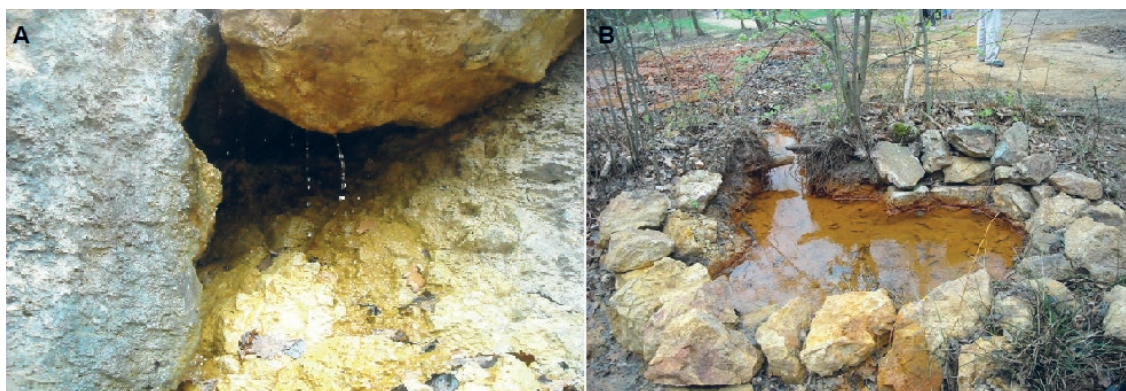
Figure 7. A- Devil's Water; B- Red Spring.
