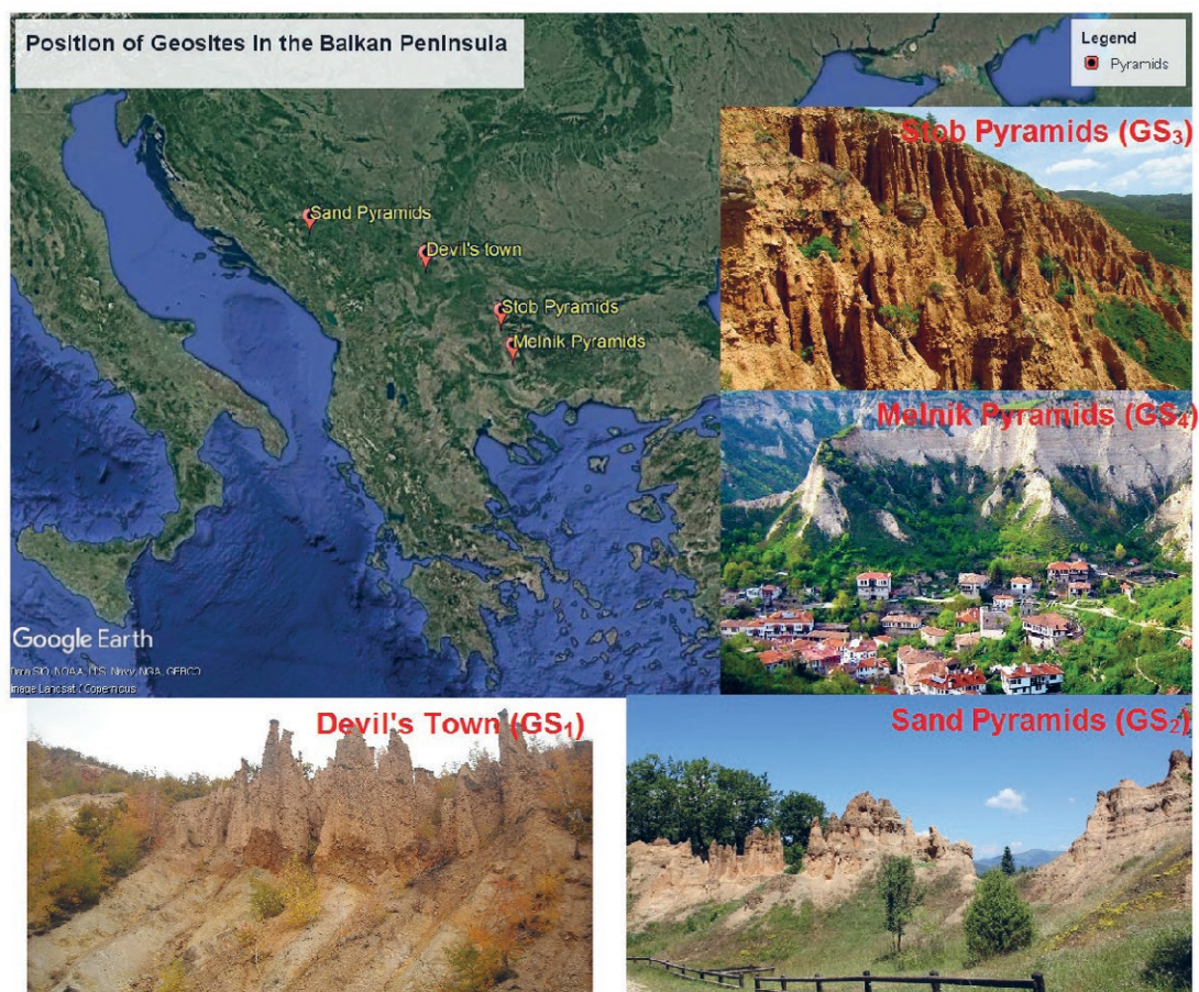
Figure 8. Position of geosites on the Balkan Peninsula.
