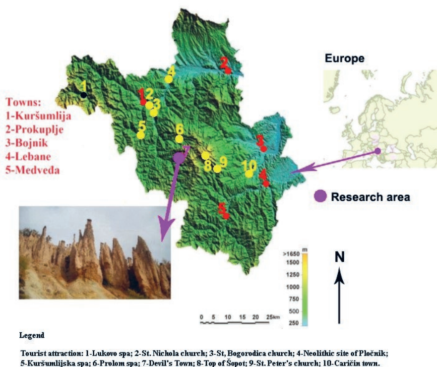
Figure 1. Location map of Devil's Town (Source of hypsometry: CGIAR Consortium for Spatial Information, 2017).
