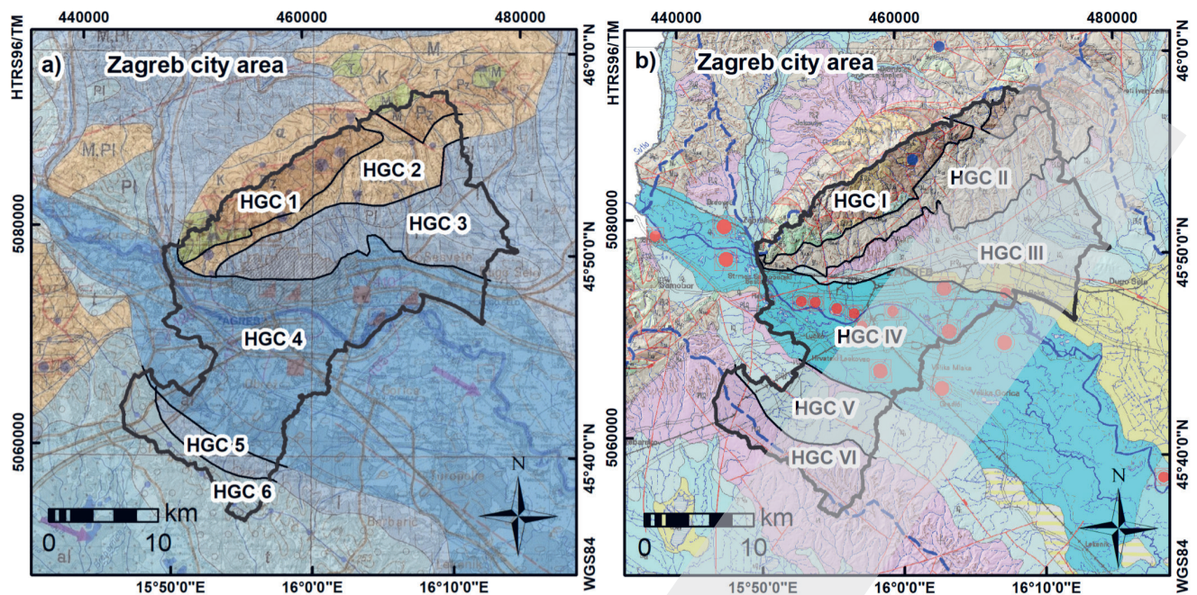
Figure 4. Hydrogeological maps of Zagreb city area with differentiated hydrogeological complexes: a Original scale 1:500,000 (IVKOVIĆ & KOMATINA, 1980); b Original scale 1:1300,000 (BIONDIĆ et al., 2003).
