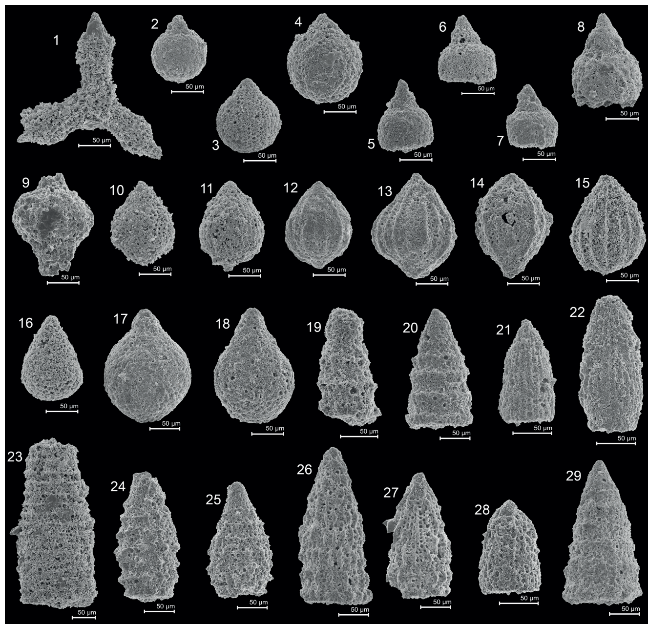
Figure 5. Middle Jurassic radiolarians from the Mala Palgruža succession. For each illustration, sample number and scanning electron micrograph number is indicated. 1 – Homoeoparonella elegans (PESSAGNO), MPV-2, MPV2_0019; 2 – Hemicryptocapsa buekkensis (KOZUR), MPZ-5, MPZ5_0032; 3 – Hemicryptocapsa nonaginta O'DOGHERTY, GORIČAN & GAWLICK, MPS-5, MPZ5_0015; 4 – Hemicryptocapsa sp. cf. H. nonaginta O'DOGHERTY, GORIČAN & GAWLICK, MPZ-5, MPZ5_0022; 5–7 – Eucyrtidiellum unumaense (YAO), 5 – MPZ-5, MPZ5_0016, 6 – MPV-2, MPV2_0013, 7 – MPZ-5, MPZ5_0017; 8 – Eucyrtidiellum sp., MPS-5, MPZ5_0003; 9 – Quarticella cf. ciccionea (CHIARI, MARCUCCI, & PRELA), MPZ-5, MPZ5_0037; 10 – Quarticella sp., MPS-5, MPZ5_0009; 11 – Striatojaponocapsa synconexa O'DOGHERTY, GORIČAN & DUMITRICA, MPS-5, MPZ5_0021; 12, 13 – Unuma darnoensis KOZUR, 12 : MPZ-5, MPZ5_0026, 13 : MPZ-5, MPZ5_0019; 14 – Unuma sp. cf. U. typicus YAO, MPZ-5, MPZ5_0036; 15 – Protunuma turbo MATSUOKA, MPV-2, MPV2_0010; 16 – Praewilliriedellum sp., MPV-2, MPV2_0024; 17, 18 – Praewilliriedellum convexum (YAO), 17 – MPZ-5, MPZ5_0040, 18 – MPZ-5, MPZ5_0031; 19 – Stichomitra? takanoensis AITA, MPZ-5, MPZ5_0009; 20 – Mizukidella kamoensis (MIZUTANI & KIDO), MPZ-5, MPZ5_0027; 21 – Archaeodictyomitra patricki KOCHER, MPZ-5, MPZ5_0004; 22 – Archaeodictyomitra sp., MPZ-5, MPZ5_0006; 23 – Parvicingulid gen. et sp. indent., MPS-5, MPZ5_0019; 24, 25 – Eoxitus baloghi KOZUR, 24 – MPZ-5, MPZ5_0012, 25 – MPZ-5, MPZ5_0035; 26 – Transhsuum brevicostatum (OŽVOLDOVA), MPZ-5, MPZ5_0008; 27 – Transhsuum maxwelli (PESSAGNO), MPZ-5, MPZ5_0034; 28 – Parahsuum sp., MPZ-5, MPZ5_0033; 29 – Canoptum krahsteineense (SUZUKI & GAWLICK), MPZ-5, MPZ5_0011.
