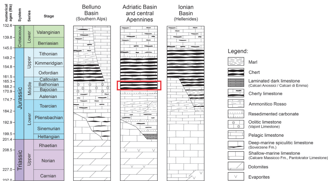
Figure 6. Chronostratigraphic overview of the Upper Triassic to lowermost Cretaceous formations of the Belluno Basin, the Ionian Basin, and the Adriatic Basin (which is similar to the Umbria–Marche basin of the central Apennines). For details and references, see text. The red rectangle marks the range of the investigated Mala Palagruža formation.
