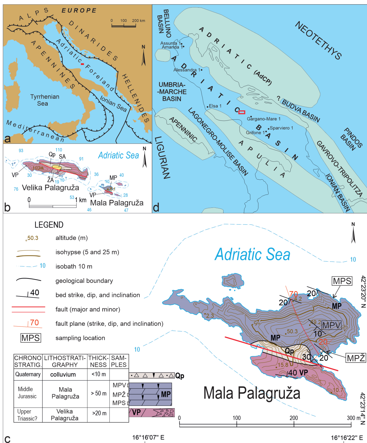
Figure 1. (a) Location map of the Palagruža archipelago in the central Adriatic (red rectangle), and the present-day regional peri-Adriatic tectonic setting (KORBAR, 2009); (b) A geological map of the Palagruža archipelago (from KORBAR et al., 2012), representing exclusive outcrops of the Mid-Adriatic Ridge; (c) A geological map of the Mala Palagruža islet and position of the sampled locations (arrows); (d) The paleogeographic position of the Palagruža archipelago during the Middle Jurassic in the central Adriatic Basin (red rectangle) showing a conservative configuration of the peri-Adriatic carbonate platforms and the surrounding basins. Black dots mark selected boreholes (see text).
