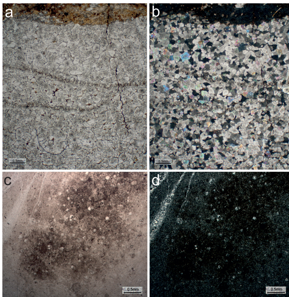
Figure 4. (a, b) Photomicrographs of a contact of microcrystalline partly siliceous dolomite (lower part) and chert (on top), with (left) and without polarizer (right). Sampling locality MPV; (c, d) Photomicrographs of amorphous chert, with (left) and without polarizer (right). Tiny, rounded spheres are probably diagenetic relicts of radiolarians. Sampling locality MPŽ.
