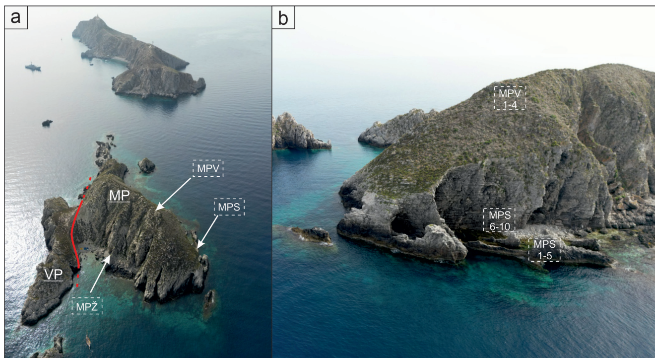
Figure 2. (a) A panoramic photograph from the east to the islet of Mala Palagruža, (Velika Palagruža is in the background on the west), with interpretation of the main geological elements and the sampling locations MPS, MPŽ and MPV. VP – Velika Palagruža formation, MP – Mala Palagruža formation; (b) A panoramic photograph from the north, showing a typical thin-bedded pelagic succession of the Mala Palagruža formation exposed on the northern cliff of the islet and the sampling locations.
