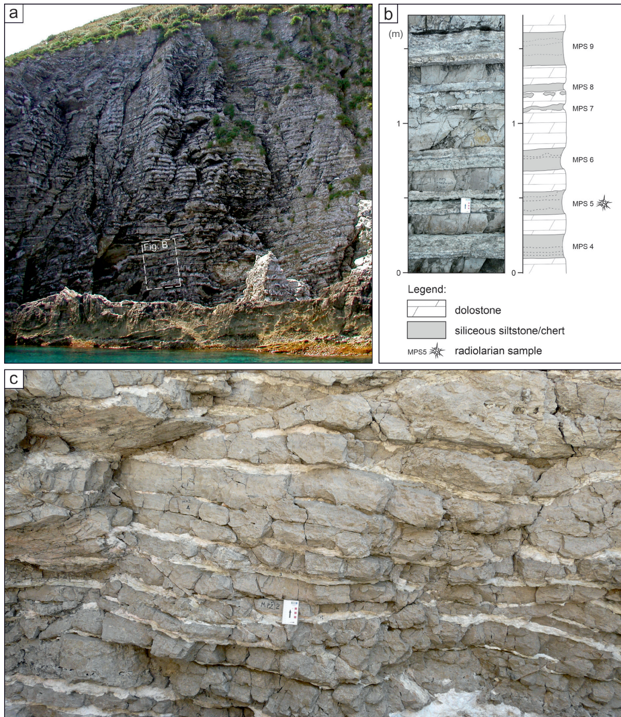
Figure 3. (a) A typical succession of the Mala Palagruža formation on the northern cliff of the islet and a schematic drawing of decimetric alternation of dolomite and chert; (b) Sampling points on the MPS location in the lower part of the Mala Palagruža succession (location marked by a rectangle on (a); (c) Sampling point Mala Palagruža žalo (MPŽ, location on Figs. 1c, 2a) that is characterized by a metre thick very thin-bedded succession bounded by two small faults.
