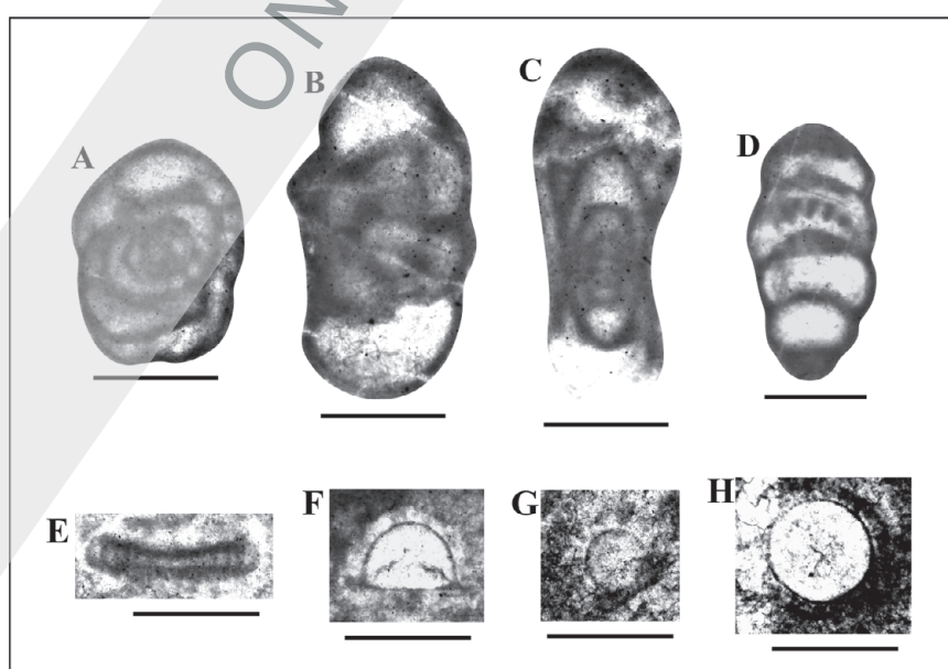
Figure 11. Photomicrographs of the foraminiferal taxa from samples 21-EL-06 of middle Viséan age and 21-EL-41 of early Serpukhovian age. A – Dainella callosa VDOVENKO in BRAZHNKOVA & VDOVENKO, 1973, 21-EL-41; B – Pojarkovella ? sp. 1, 21-EL-41; C – Millerella sp. 1, 21-EL-41; D – Haplophragmella sp. 1, 21-EL-41; E – Hemidiscopsis muradymica (KULAGINA in KULAGINA et al., 1992), 21-EL-06; F – Eotuberitina sp., 21-EL-06; G–H – Radiosphaera sp., G – 21-EL-06, H – 21-EL-06. Scale bar for A–C and E–H is 0.25 mm and for D is 0.5 mm.
