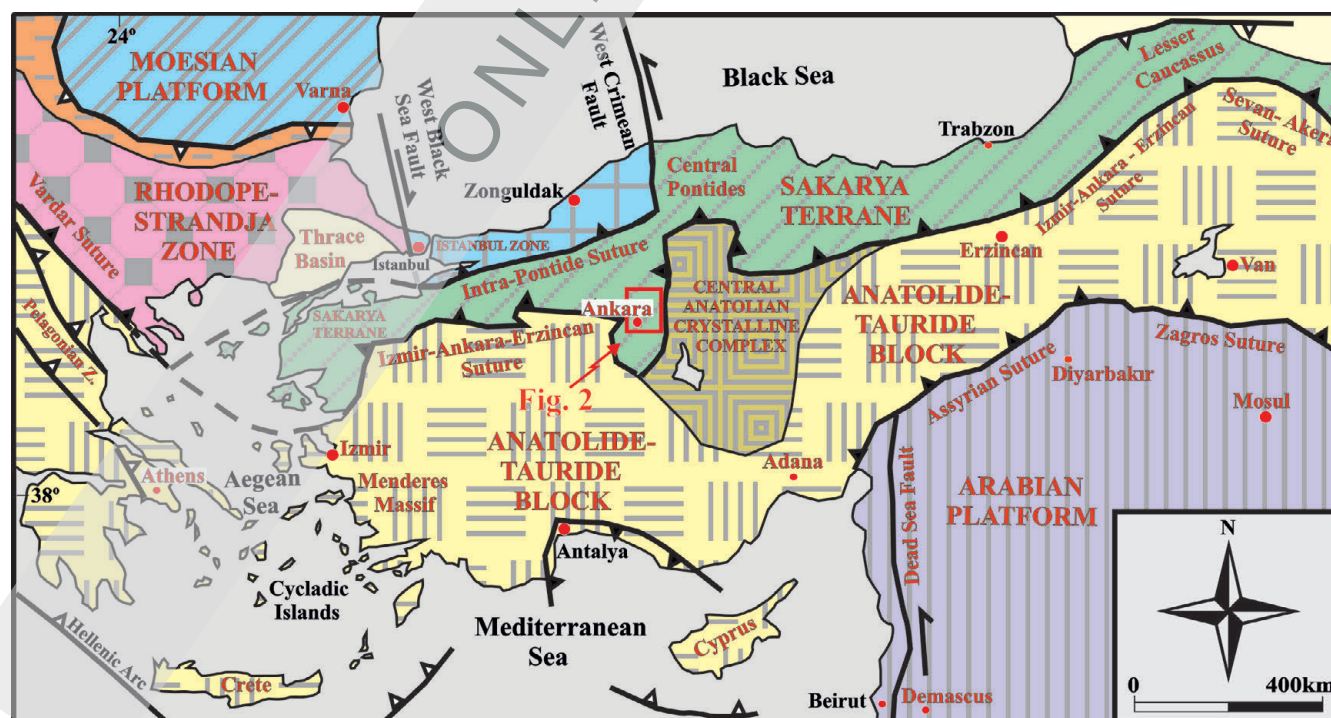
Figure 1. Tectonic map of Türkiye and its surroundings with major suture zones/terrane and location of the studied region around Ankara city (slightly revised after OKAY & TÜYSÜZ, 1999; OKAY & GÖNCÜOĞLU, 2004).
