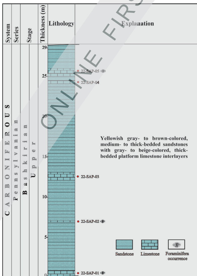
Figure 9. Log of the Sapankiran section and sampling levels.
