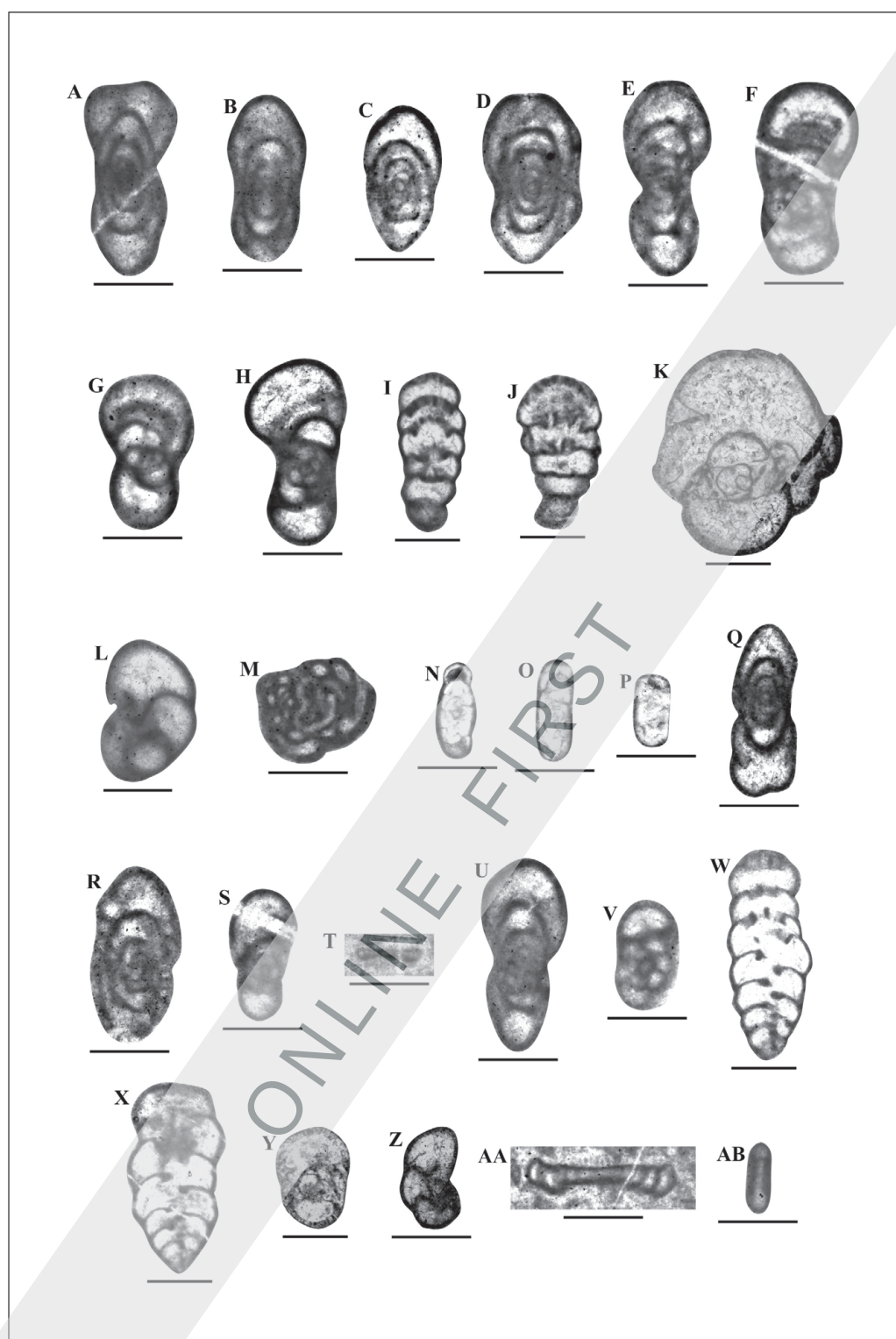
Figure 12. Photomicrographs of the foraminiferal taxa from the Neoarchaediscus postrugosus - Biseriella parva Assemblage Zone in the Kapakli section of early Serpukhovian age; A – Eostaffella ex gr. pseudostruvei (RAUZER-CHERNOUSOVA & BELYAEV, in RAUZER-CHERNOUSOVA et al., 1936), 22-KPK-04; B – Eostaffella acutiformis KIREEVA in RAUZER-CHERNOUSOVA et al., 1951, 22-KPK-04; C – Eostaffella cf. proikensis RAUZER-CHERNOUSOVA, 1948, 22-KPK-04; D – Eostaffella chusovensis acutiformis KIREEVA in RAUZER-CHERNOUSOVA et al., 1951, 22-KPK-04; E – Millerella paraumbilicata MANUKALOVA-GREBENYUK, ILYINA & SEREZHNKOVA in MANUKALOVA-GREBENYUK et al., 1969, 22-KPK-04; F – Endothyra demini DURKINA, 1959, 22-KPK-04; G – Endothyra karasikae DURKINA, 1959, 22-KPK-04; H – Planoendothyra aljutovica (REITLINGER, 1950), 22-KPK-04; I – Haplophragmella irregularis RAUZER-CHERNOUSOVA, 1938, 22-KPK-04; J – Haplophragmella sp. 2, 22-KPK-04; K – Janischewskina orbiculata (GANELINA, 1956), 22-KPK-04; L – Biseriella parva (CHERNYSHEVA, 1948), 22-KPK-04; M – Pseudoglomospira sp. 1, 22-KPK-04; N – Neoarchaediscus postrugosus (REITLINGER, 1949), 22-KPK-04; O – Neoarchaediscus parvus (RAUZER-CHERNOUSOVA, 1948), 22-KPK-04; P – Neoarchaediscus sp. 1, 22-KPK-04; Q – Eostaffella ex gr. pseudostruvei (RAUZER-CHERNOUSOVA & BELYAEV in RAUZER-CHERNOUSOVA et al., 1936), 22-KPK-05; R – Eostaffella ex gr. postproikensis VDOVENKO in BRAZHNKOVA et al., 1967, 22-KPK-05; S – Mediendothyra aff. angusta (DURKINA, 1959), 22-KPK-05; T – Eolasiodiscus ? sp. 1, 22-KPK-05; U – Millerella marblensis THOMPSON, 1942, 22-KPK-06; V – Granuliferella minima (LIPINA, 1955), 22-KPK-06; W – Koskinobigenerina sp. 1, 22-KPK-06; X – Koskinobigenerina sp. 2, 22-KPK-06; Y – Bradyina sp. 1, 22-KPK-06; Z – Biseriella sp. 1, 22-KPK-06; AA – Hemidiscopsis sp. 1, 22-KPK-06; AB – Mediocris breviscula subsp. celsa POYARKOV, 1965, 22-KPK-06. Scale bar for A–C, E–L, Q–Z is 0.25 mm and for D, M–P, AA–AB is 0.5 mm.
