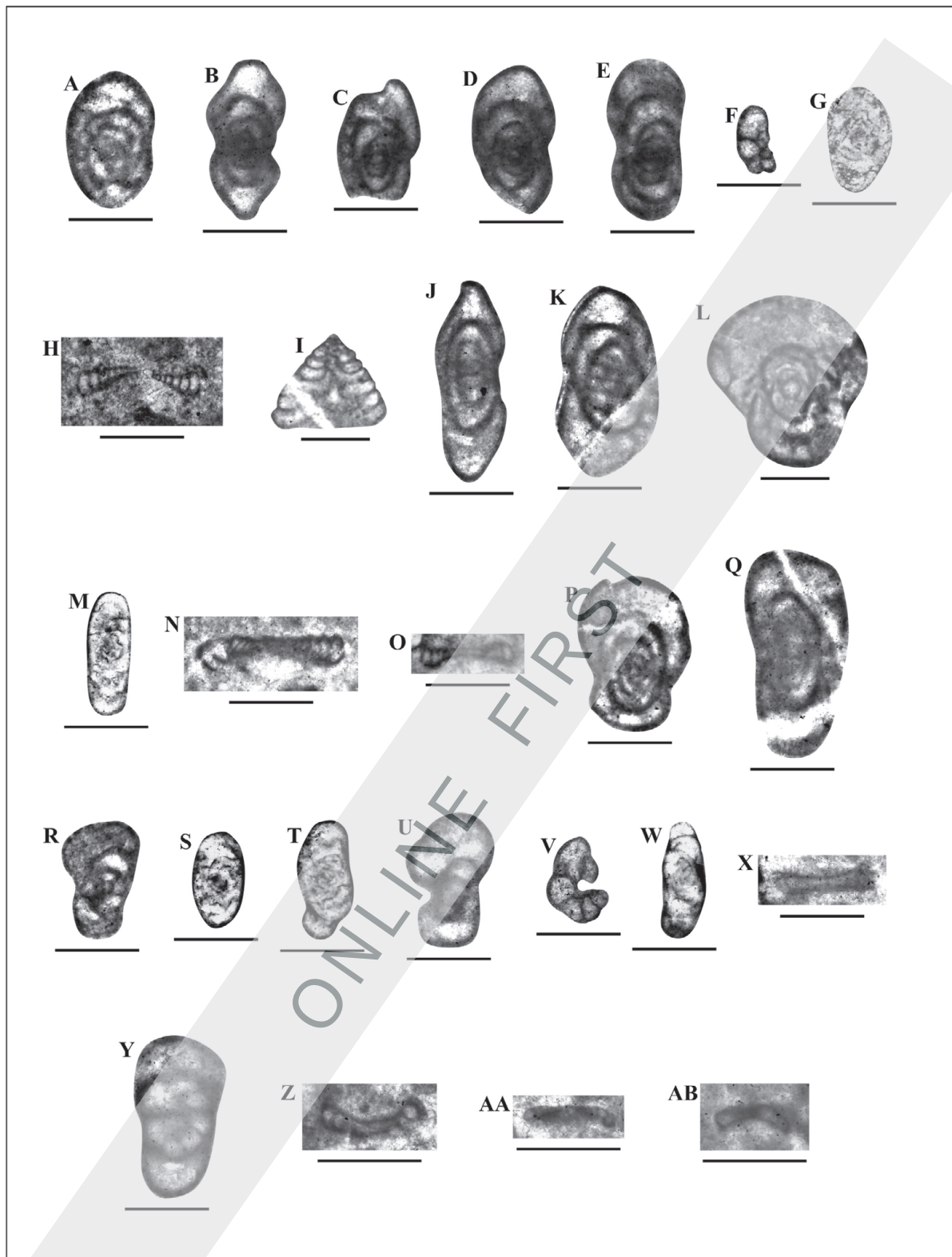
Figure 15. Photomicrographs of the foraminiferal taxa from the Eostaffellina decurta Zone and Eostaffellina paraprotvae Zone in the Kapaklı section of early late-late Serpukhovian age. A – Praeostaffellina macdonaldensis CÓZAR et al., 2008b, 22-KPK-10; B – Eostaffella acutiformis KIREEVA in RAUZER-CHERNOUSOVA et al., 1951, 22-KPK-10; C–D – Eostaffellina decurta (RAUZER-CHERNOUSOVA, 1948), both from 22-KPK-10; E – Eostaffellina sp. 1, 22-KPK-10; F – Biseriella sp. 2, 22-KPK-10; G – Brenckleina sp. 1, 22-KPK-10; H – Turrispiroides sp. 1, 22-KPK-10; I – Tetrataxis conica EHRENBERG, 1854, 22-KPK-10; J – Eostaffella ex gr. pseudostrovei (RAUZER-CHERNOUSOVA & BELYAEV in RAUZER-CHERNOUSOVA et al., 1936), 22-KPK-11; K – Eostaffella ex gr. postproikensis VDOVENKO in BRAZHNIKOVA et al., 1967, 22-KPK-11; L – Janischewskina sp. 2, 22-KPK-11; M – Neoarchaediscus gregorii (DAIN in DAIN & GROZDILOVA, 1953), 22-KPK-11; N – Monotaxinoides sp. 1, 22-KPK-11; O – Monotaxinoides sp. 2, 22-KPK-11; P – Eostaffellina paraprotvae (RAUZER-CHERNOUSOVA, 1948), 22-KPK-12; Q – Endothyranopsis compressa subsp. plana BRAZHNIKOVA in BRAZHNIKOVA et al., 1967, 22-KPK-12; R – Endothyra sp. 1, 22-KPK-12; S – Brenckleina sp. 2, 22-KPK-12; T – Neoarchaediscus sp. 2, 22-KPK-12; U – Endothyra sp. 1, 22-KPK-13; V – Biseriella sp. 2, 22-KPK-13; W – Neoarchaediscus bykovensis SOSIPATROVA, 1966, 22-KPK-13; X – Monotaxinoides sp. 2, 22-KPK-13; Y – Endothyra similis RAUZER-CHERNOUSOVA & REITLINGER in RAUZER-CHERNOUSOVA et al., 1936, 22-KPK-14; Z–AB – Howchinia subplana (BRAZHNIKOVA & YARTSEVA, 1956), all from 22-KPK-14. Scale bar for A–H, J–K, M–AB is 0.25 mm and for I and L is 0.5 mm.
