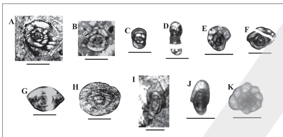
Figure 16. Photomicrographs of the foraminiferal taxa from the Sapankiran section. A–B – Staffellaformes bona (GROZDILOVA & LEBEDEV, 1954), both from 22-SAP-01; C – Semistaffella cf. minuscilaria (REITLINGER in KULAGINA, 1988), 22-SAP-01; D – Eostaffella sp. A, 22-SAP-01; E – Schubertella sp., 22-SAP-01; F–G – Staffellaformes parva (LEE & CHEN in LEE et al., 1930), both from 22-SAP-02; H – Staffellaformes cf. staffellaformis (KIREVA in RAUZER-CHERNOUSOVA et al., 1951), 22-SAP-02; I – Millerella? sp., 22-SAP-05; J – Eostaffella sp. B, 22-SAP-05; K – Endothyra sp., 22-SAP-05. Scale bar for A–D, F–H is 0.5 mm and for E, I–K is 0.25 mm.
