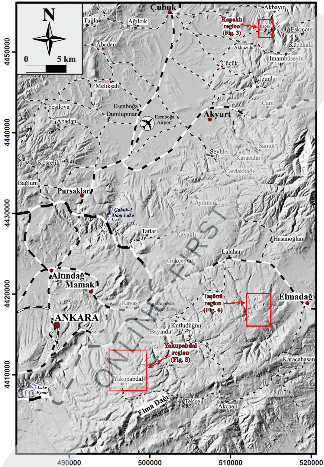
Figure 2. Location map showing the distribution of the studied regions (Kapaklı, Taşönü, and Yakupabdal) around Ankara city.
