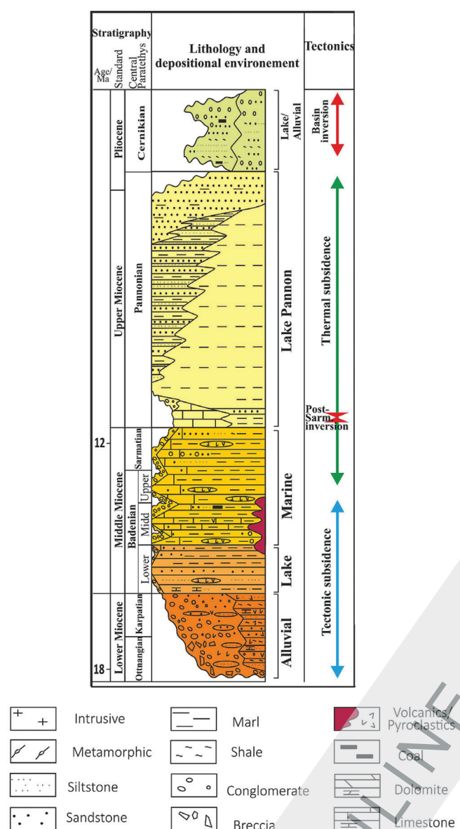
Figure 2. Stratigraphy, lithology, and depositional environment of the Neogene of the North Croatian Basin (modified from RUKAVINA et al., 2023 and PAVELIĆ & KOVAČIĆ, 2018).
