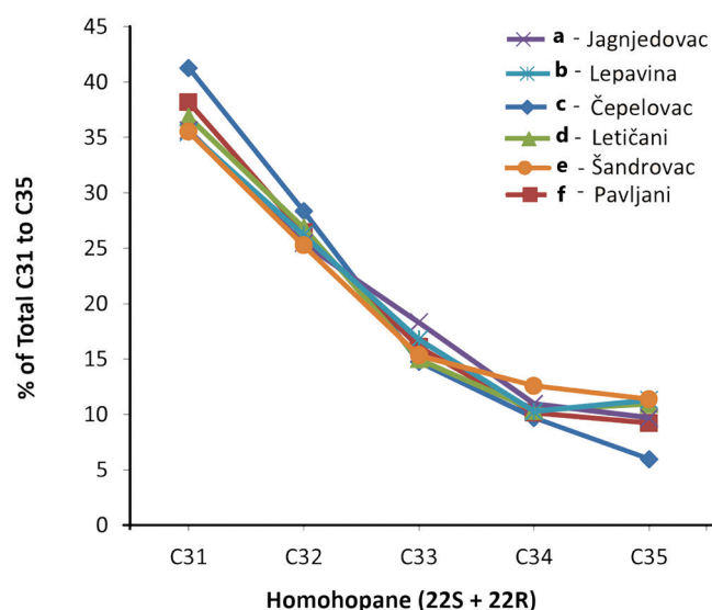
Figure 7. Distributions of C_{31} – C_{35} \alpha\beta homohopanes of the investigated oils: a – Jagnjedovac; b – Lepavina; c – Čepelovac; d – Letičani; e – Šandrovac; f – Pavljani.
