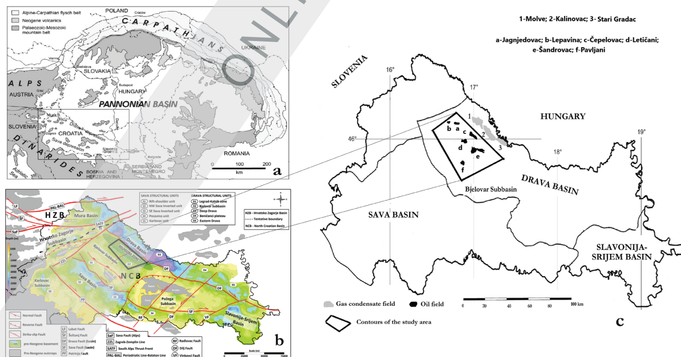
Figure 1. (a) Pannonian Basin; (b) Classification of structures and faults of the Croatian part of the Pannonian Basin (modified from TROSKOT-ČORBIĆ et al., 2026); (c) Locations of samples in the study area, Oils: a – Jagnjedovac; b – Lepavina; c – Čepelovac; d – Letičani; e – Šandrovac; f – Pavljani; Gas-condensates: 1 – Molve; 2 – Kalinovac; 3 – Stari Gradac (modified from BARIĆ et al., 2000).
