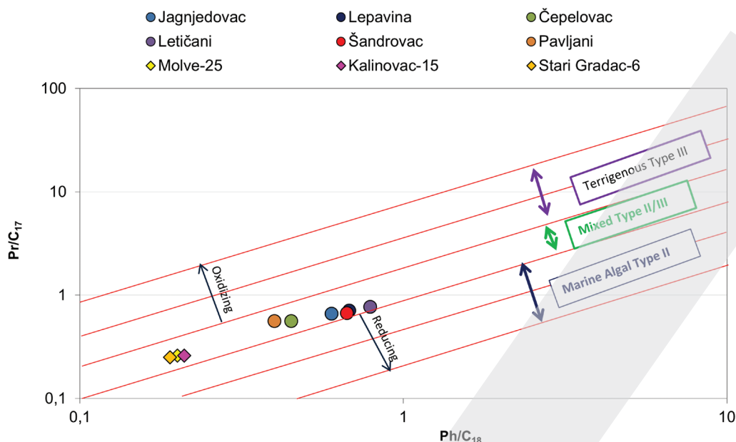
Figure 4. Pr/nC_{17} versus Ph/nC_{18} plot of investigated oils and gas-condensates (SHANMUGAM, 1985). Pr – pristine, Ph – phytane.
