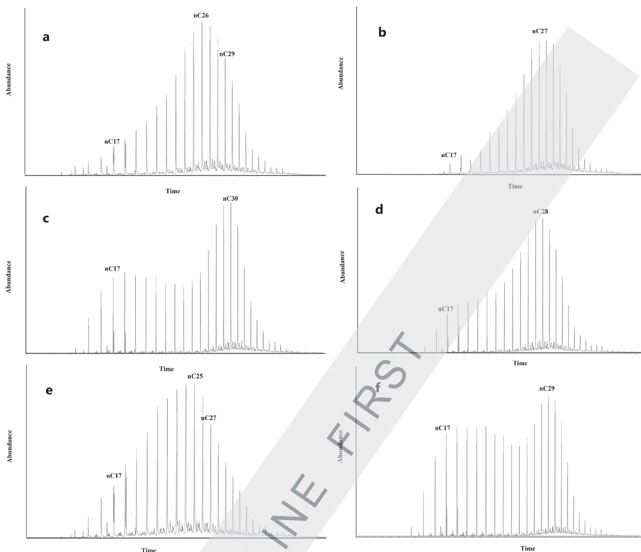
Figure 3. Mass fragmentograms of n -alkanes ( m/z = 85 ) of investigated oils: a – Jagnjedovac; b – Lepavina; c – Čepelovac; d – Letičani; e – Šandrovac; f – Pavljani.
