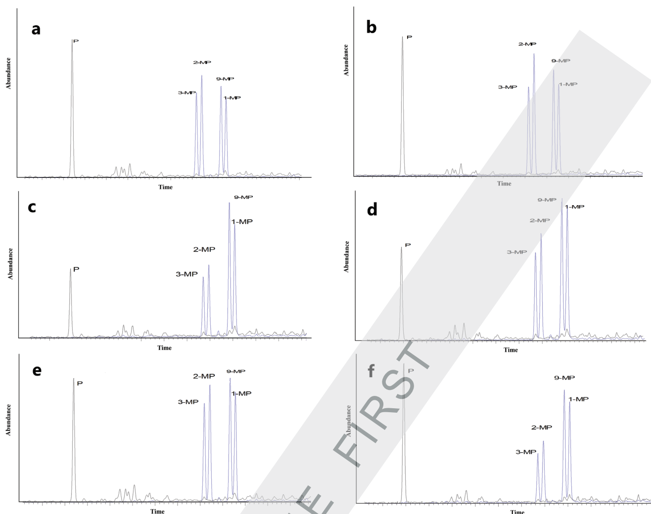
Figure 10. Mass chromatograms of phenanthrene and methylphenanthrenes ( m/z = 178 + 192 ) of the investigated oils: a – Jagnjedovac; b – Lepavina; c – Čepelovac; d – Letičani; e – Šandrovac; f – Pavljani. P – phenanthrene; MP – methylphenanthrene.
