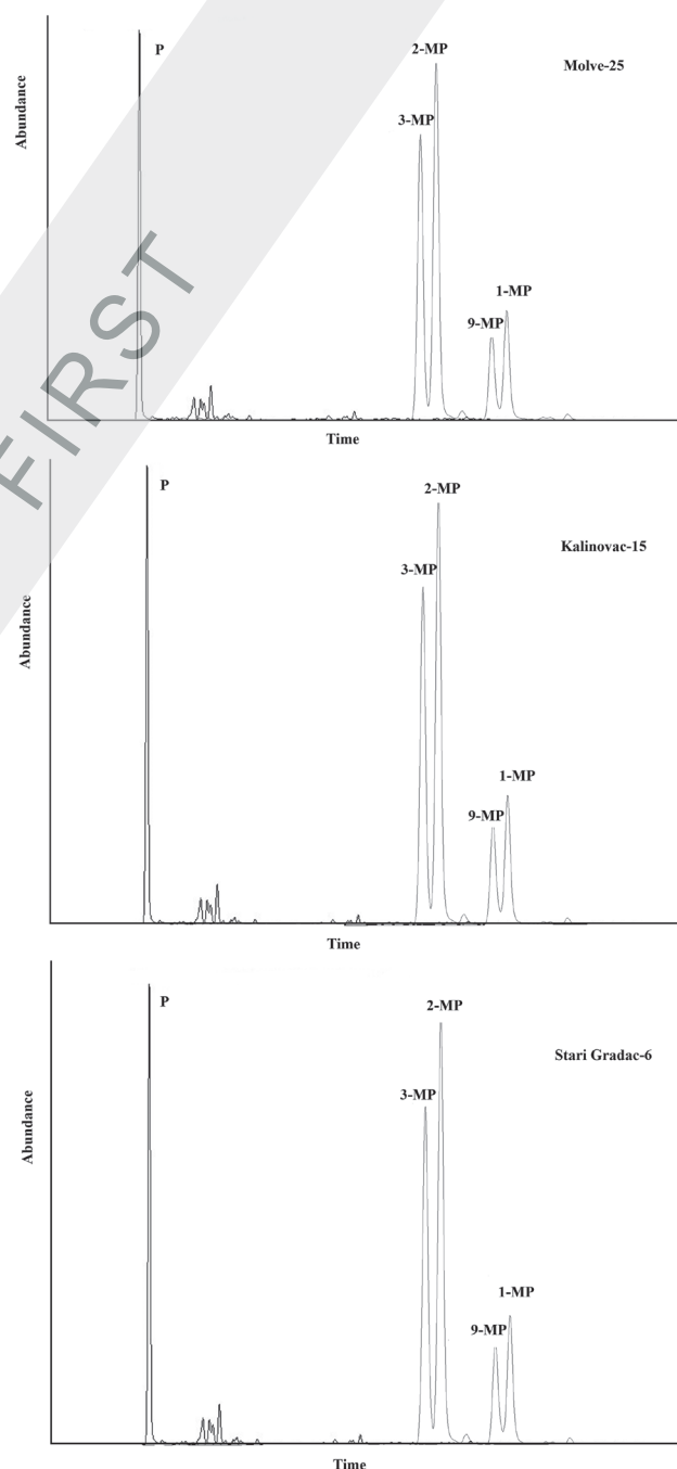
Figure 11. Mass chromatograms of phenanthrene and methylphenanthrenes ( m/z = 178 + 192 ) of the gas-condensates Molve-25, Kalinovac-15 and Stari Gradac-6. P – phenanthrene; MP – methylphenanthrene.
