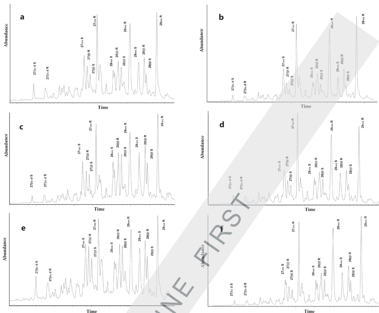
Figure 5. Mass chromatograms of steranes ( m/z = 217 ) of the investigated oils: a – Jagnjedovac; b – Lepavina; c – Čepelovac; d – Letičani; e – Šandrovac; f – Pavljani. Identification is given in Table 3.
