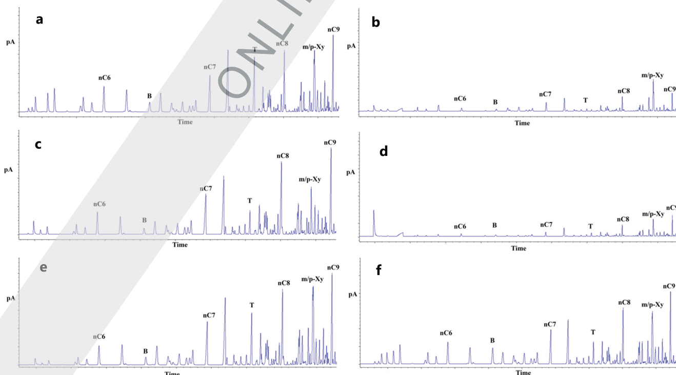
Figure 8. Gasoline fractions of the investigated oils: a – Jagnjedovac; b – Lepavina; c – Čepelovac; d – Letičani; e – Šandrovac; f – Pavljani. nC6 – n -hexane; B – benzene; nC7 – n -heptane; T – toluene; nC8 – n -octane; m/p-Xy – meta/para-xylene; nC9 – n -nonane.
