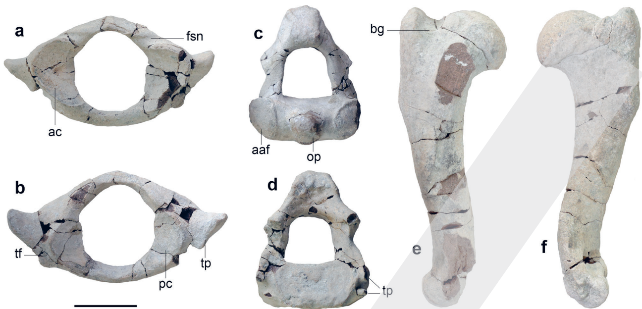
Figure 5. Referred vertebrae and humerus of Prototherium transylvanicum n. sp. (a, b) atlas (UBB V. 1153); (c, d) axis (UBB V. 1154); (e, f) right humerus (UBB V. 1157). a, c – anterior views, b, d – posterior views, e – medial view; f – lateral view. Abbreviations: aaf – anterior articular facet, ac – anterior cotyle, bg – bicipital groove, fsn – passage of first spinal nerve, op – odontoid process, pc – posterior cotyle, tf – transverse foramen, tp – transverse process. Scale bar = 3 cm.
