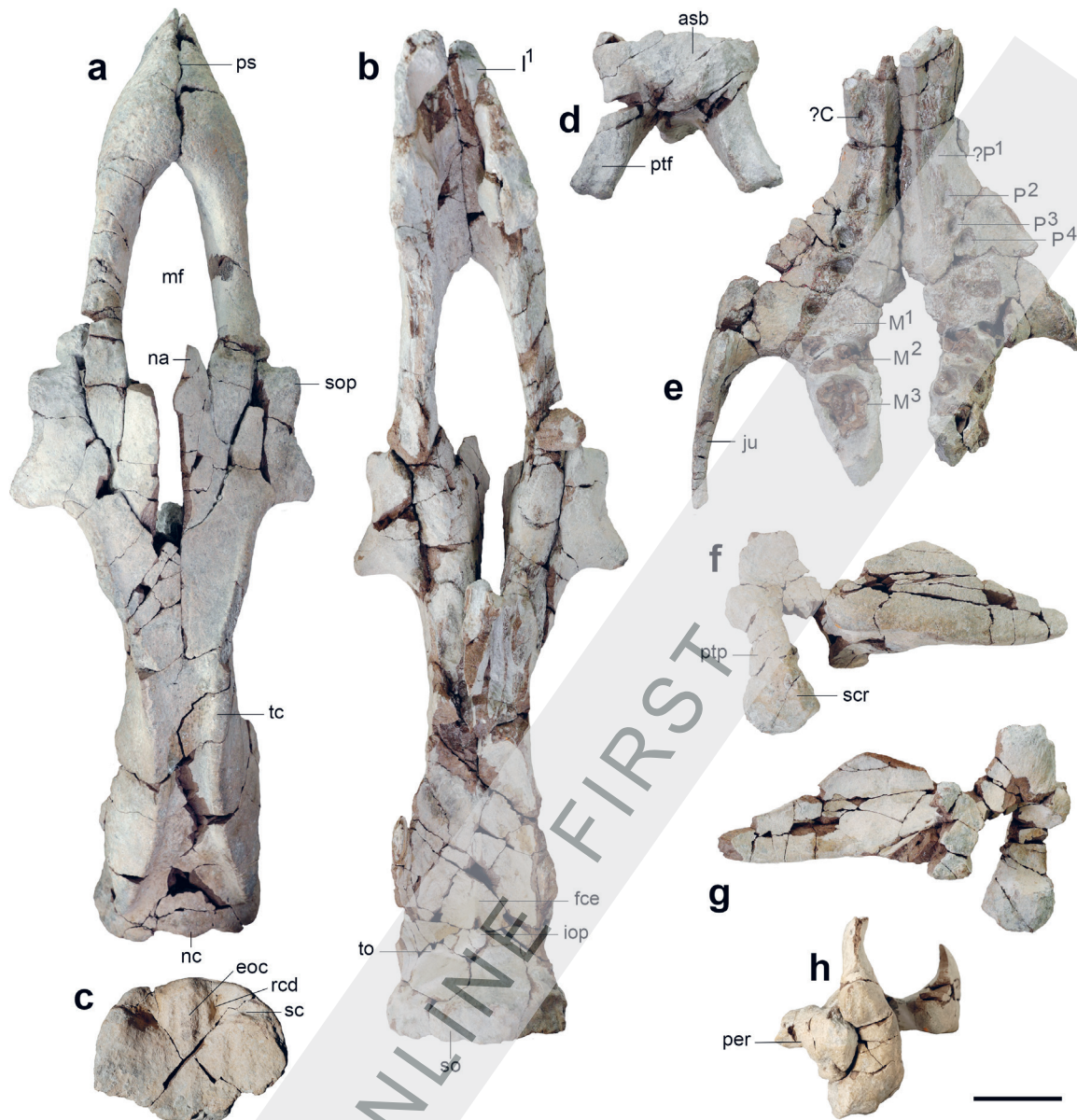
Figure 3. Referred partial skull (UBB V. 1149) and isolated cranial bones of Prototherium transylvanicum n. sp. ( a , b ) partial skull roof; ( c ) supraoccipital; ( d ) sphenopalatine (UBB V. 1152); ( e ) paired maxillae and right jugal (UBB V. 1150); ( f , g ) right squamosal; ( h ) right squamosal and right periotic (UBB V. 1151). a – dorsal view, b , e – ventral views, c , d , h – posterior views, f – lateral view, g – medial view. Abbreviations: asb – articular surface with basioccipital, C – canine, eoc – external occipital crest, fce – falx cerebri, l – incisive, iop – internal occipital protuberance, ju – jugal, M – upper molar, mf – mesorostral fossa, na – nasal, nc – nuchal crest, P – premolar, per – periotic, ptf – pterygoid fossa, ptp – post-tympanic process, rcd – insertion surface for rectus capitis dorsalis muscle, sc – insertion surface for semispinalis capitis muscle, scr – sigmoid crest, so – supraoccipital, sop – supraorbital process, tc – temporal crest, to – tentorium osseum. Scale bar = 3 cm.
