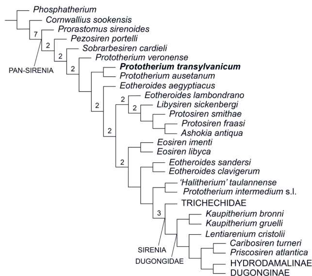
Figure 6. Relationships of Prototherium transylvanicum n. sp., based on parsimony analysis. Shortest most parsimonious tree generated by TNT, based on 63 operational taxonomic units with 89 phenotypic characters, derived from DÍAZ-BERENGUER et al. (2022). The numbers above the nodes indicate the decay indices of Bremer (= extra steps).
