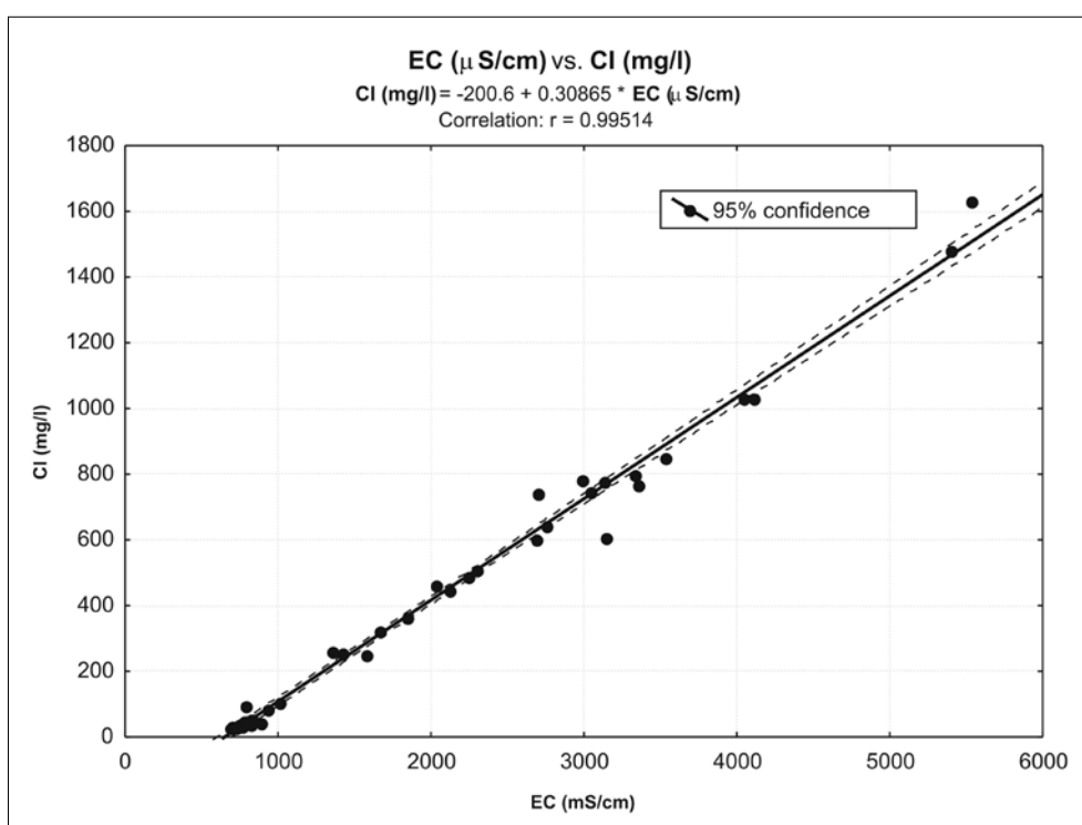
Fig. 7 Correlation between chlorides and electrolytic conductivity at the Golubinka spring.
