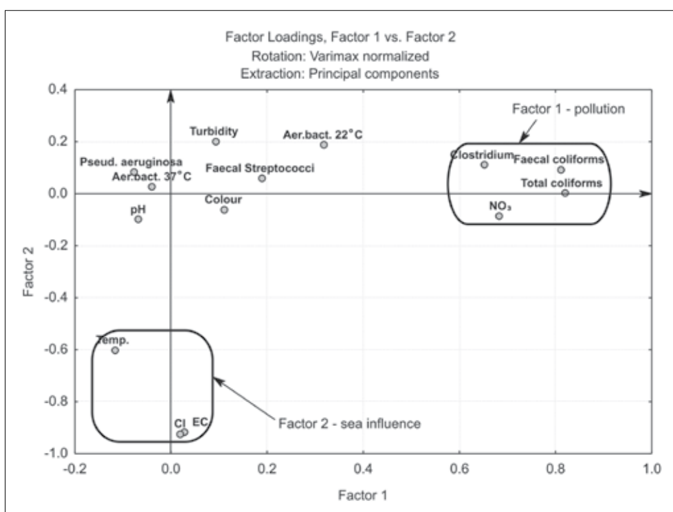
Fig. 8 Multivariate factor analysis diagram. Factor loadings: Factor 1 vs. Factor 2.
